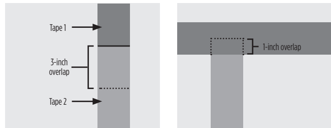
Detail G - Shingle fashion technique
