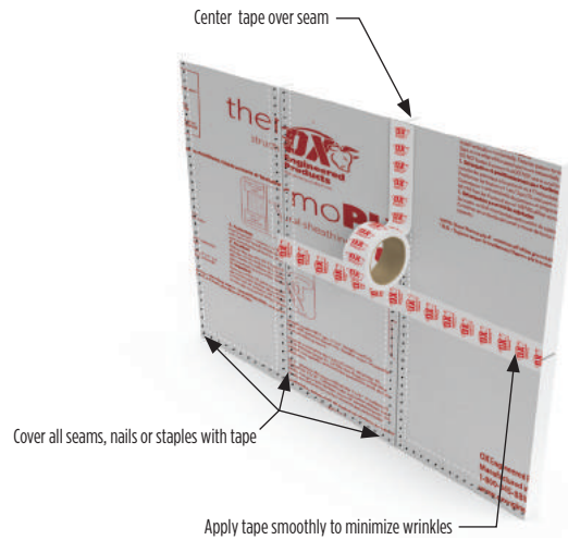
Detail F
