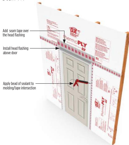
Detail M
