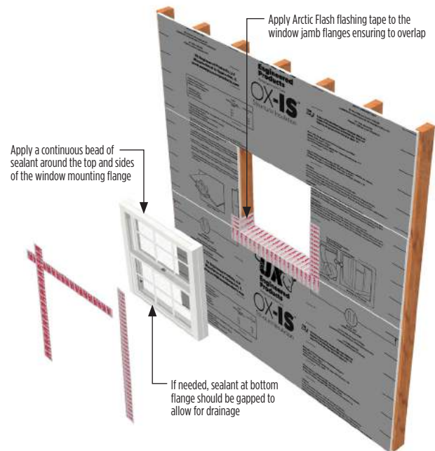
Detail G
