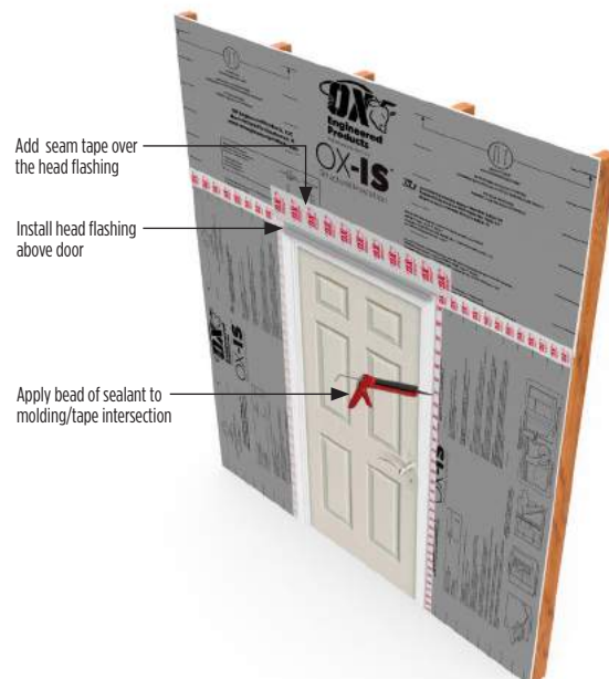
Detail J
