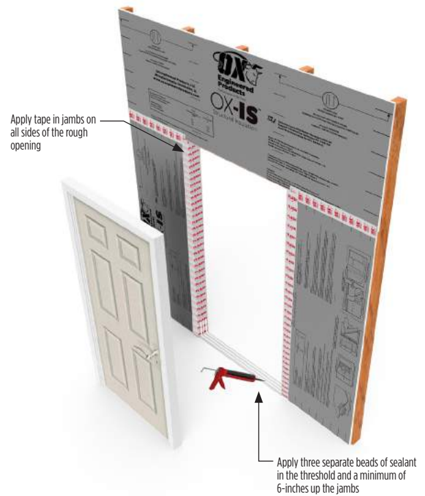
Detail J
