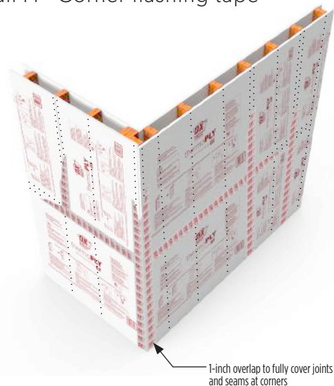
Detail H - Corner flashing tape
