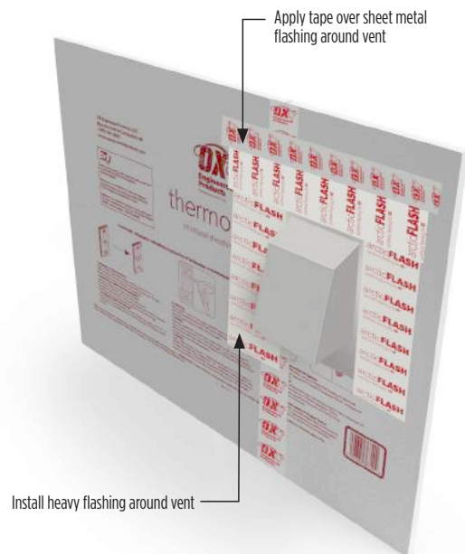
Detail O - Completed installation
