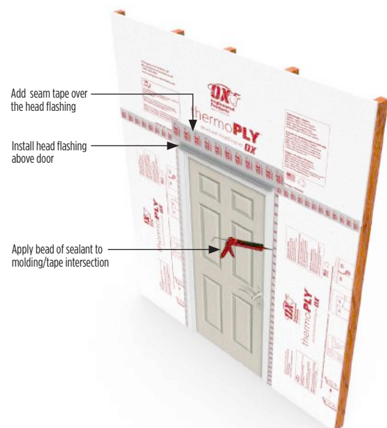
Detail L
