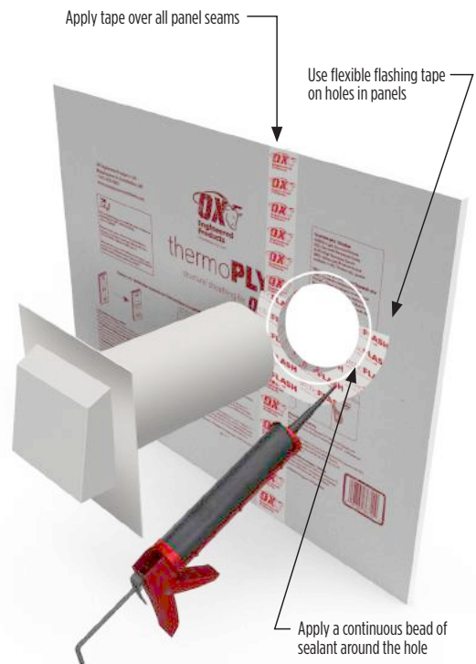
Detail O - Completed installation
