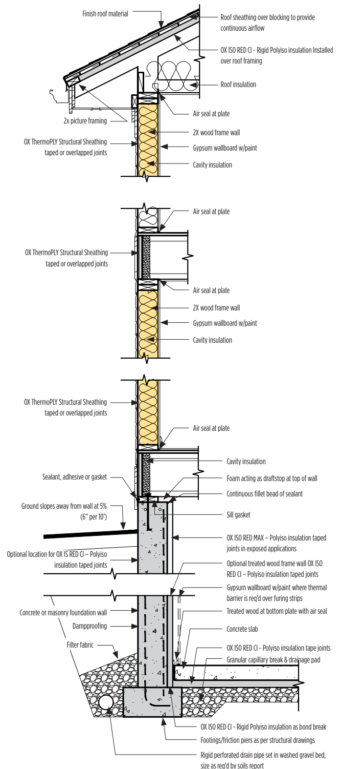
Detail A
