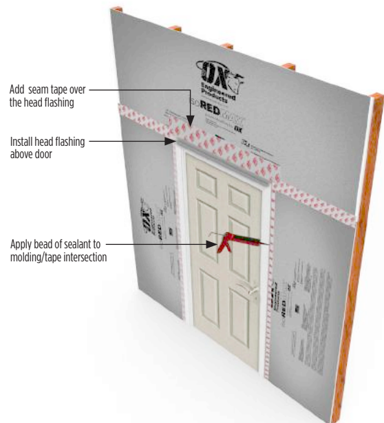
Detail L
