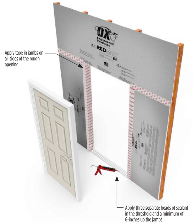
Detail L
