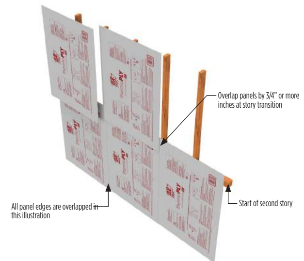
Detail C
